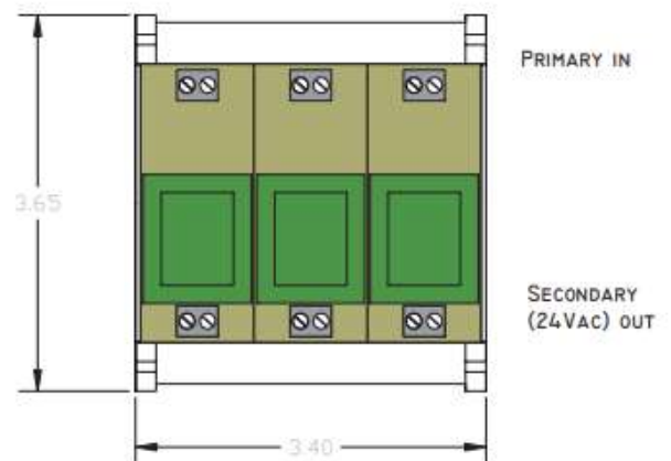
Three Phase Power Supply
