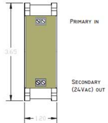
Single Phase Power Supply
