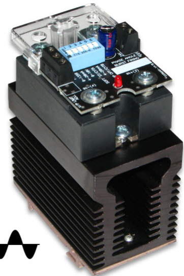
LPC A Series Proportional Output (Phase-Angle) Solid State Relay Power Controller
